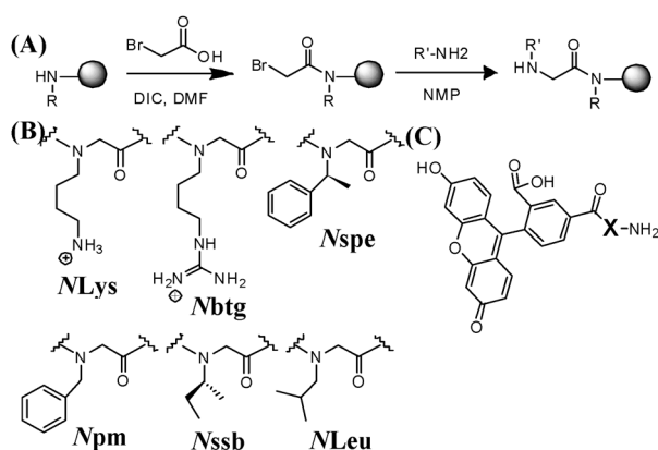
Fig. 1 The construct synthesis. (A), the submonomer synthesis scheme of peptoids; (B), peptoid monomer structures with shorthand names; (C), chemical structures of cell penetrating constructs (X) labeled with 5(6)-Carboxyfluorescein (CF).
